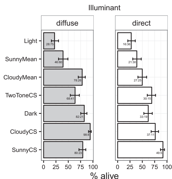
Fig. 2. Proportion surviving (mean \pm SEM) in each treatment and illumination condition (Left, diffuse; Right, direct sun). Total frequencies across all blocks are given inside the bars as numbers alive:dead. The treatments have been ordered by mean survival across illumination conditions for ease of comparison.
